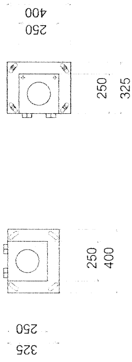
FOOTING DETAIL
